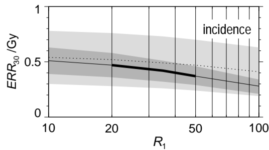
Fig. A.1: The solid line and the dark shaded band represent – for the age at exposure model – the parameter c , i.e. the ERR_{30} for solid cancer incidence due to an acute \gamma -ray dose of 1Gy and its 95%-confidence region. The broken line and the light shaded band gives the estimate of the initial slope, \alpha , and its 95%-confidence region. The diagram is analogous to the diagrams in Fig.3.
